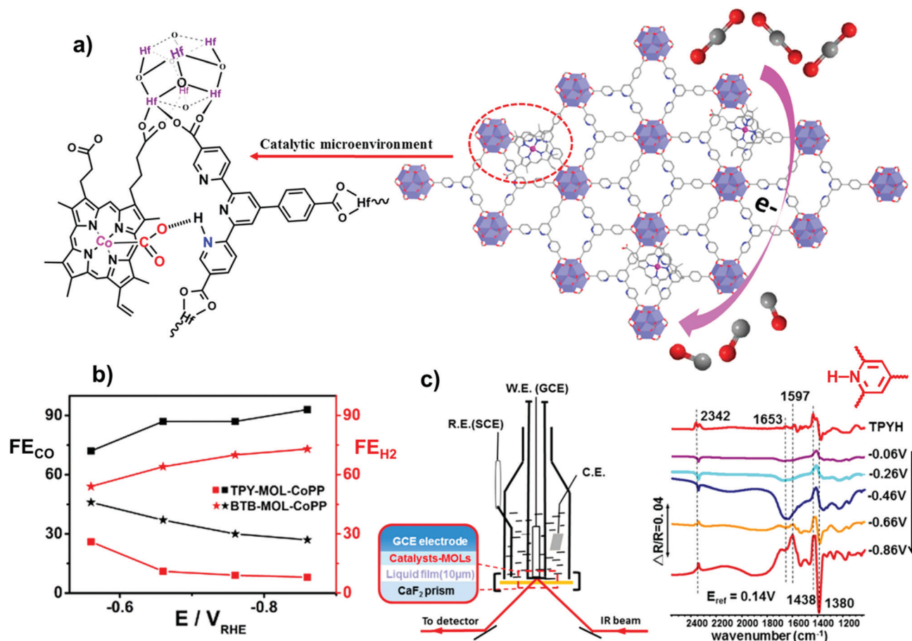
Fig. 9 (a) Schematic showing the structure of the TPY-MOL-CoPP and the cooperative activation of CO 2 by CoPP and p + H. (b) FE for CO and H 2 at varying electrolysis potentials for different catalysts in CO 2 -saturated 0.1 M NaHCO 3 . (c) On the left it is shown a schematic of the thin-layer IR cell for the in situ DRIFTS measurements. On the right, the IR spectrum of TPYH + -MOL (pH 4.0 with HClO 4 , red line), and DRIFTS of TPY-MOL-CoPP in the potential scan range of -0.06 to -0.86 V vs. RHE in a CO 2 -saturated aqueous solution of 0.1 M NaHCO 3 . The reference spectrum was taken at 0.14 V vs. RHE. Adapted with permission from ref. 168. Copyright 2019 American Chemical Society.
