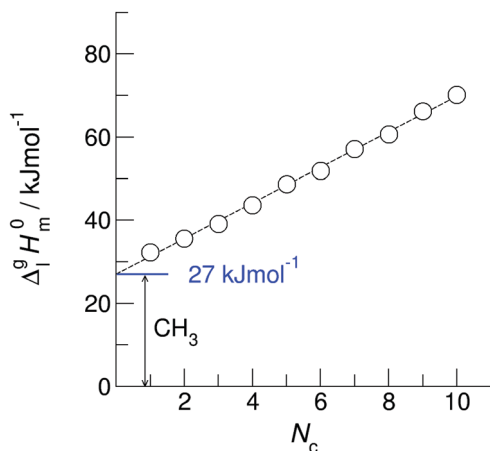
Fig. 2 Measured vaporization enthalpies, \Delta_1^e H_m^0 , of alkyl acetates plotted versus the total number of carbon atoms ( N_C ) in the side chains. The intercept of about 27 \text{ kJ mol}^{-1} at N_C = 0 gives the contribution of the \text{CH}_3 group and allows the correction of the intermolecular HB energy in aliphatic carboxylic acids. The experimental data are taken from Table 2.
