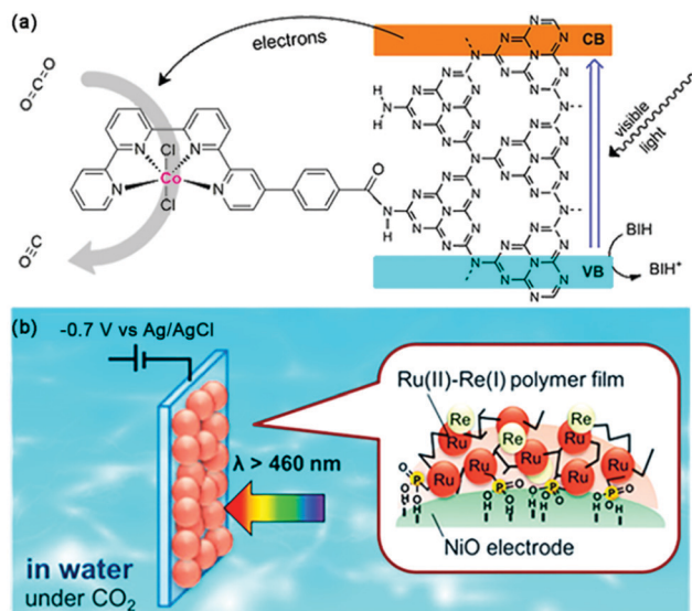
Fig. 16 (a) Visible-light-driven CO 2 reduction by a cobalt complex covalently linked to mesoporous carbon nitride. Reprinted with permission from ref. 121. Copyright 2020 American Chemical Society. (b) PolyRuRe/NiO photocathode for CO 2 photoreduction. Reprinted with permission from ref. 124. Copyright 2019 American Chemical Society.
