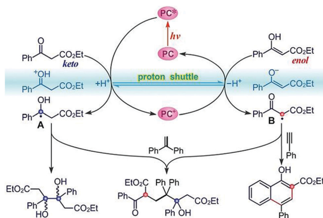
Fig. 17 Photoredox catalysis of aromatic β-ketoester for the in situ production of transient and persistent radicals for organic transformation. Reprinted with permission from ref. 126. Copyright 2020 Wiley-VCH.
