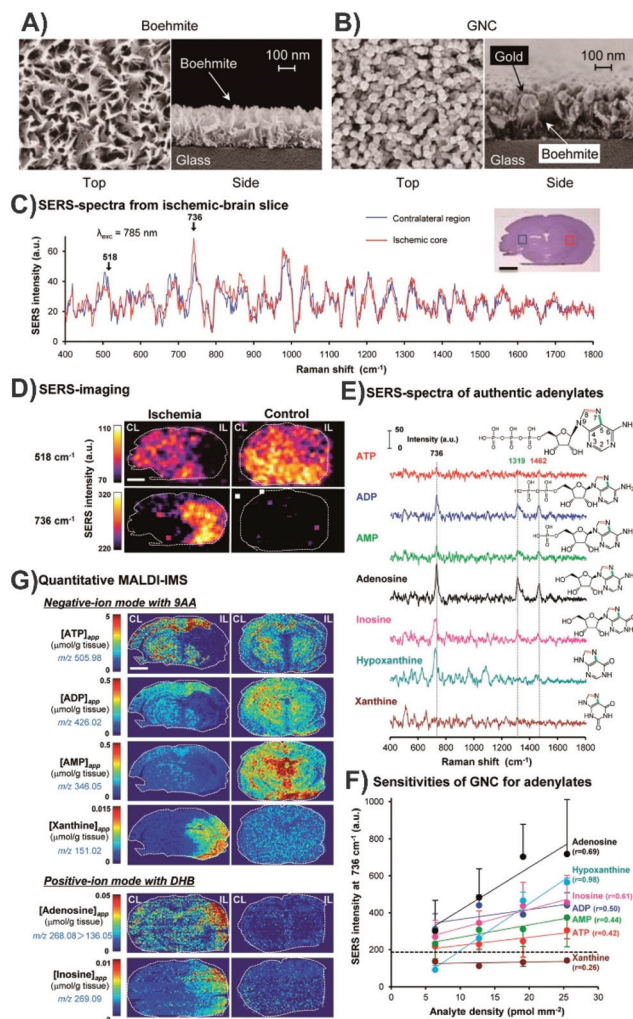
Fig. 5 SEM images of (A) boehmite and (B) gold nanocol (GNC). (C) Average SERS spectra from an ischemic core (red) and its contralateral region (blue) of an ischemic brain slice. (D) SERS maps of the bands at 518 and 736 \text{cm}^{-1} for ischemic and control brain slices. (E) SERS spectra of various adenylates. (F) Relative sensitivity of the GNC substrates to adenine related compounds. (G) Quantitative imaging mass spectrometry showing the spatial distribution of apparent tissue contents of various adenylates from tissue slices taken from the same animal as the SERS images of (D). The scale bars in the images is 2 mm. Adapted with permission from ACS Nano , 2014, 8 , 5622–5632 (ref. 83). Copyright (2014) American Chemical Society.
