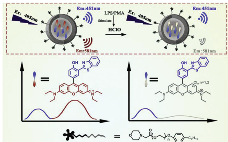
Fig. 5 Structures and mechanism for the selective visualization of lysosomal \text{HClO} by the SSRN nanoprobe. Reprinted with permission from ref. 101. Copyright 2020, Elsevier.
