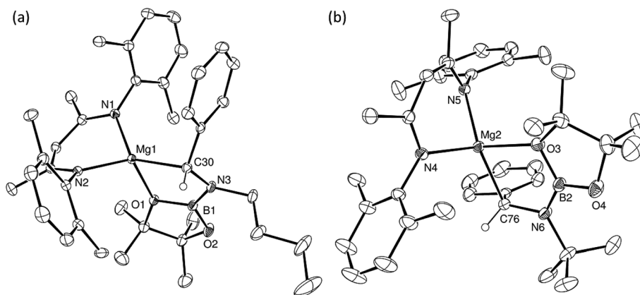
Fig. 2 ORTEP representations (25% probability ellipsoids) of (a) compound 15_{\text{BN}} and (b) the Mg2-containing molecule of compound 16_{\text{BN}} . Hydrogen atoms except for those attached to C30 ( 15_{\text{BN}} ) and C76 ( 16_{\text{BN}} ), iso-propyl methyl groups and the Mg1-containing molecule of compound 16_{\text{BN}} have been removed for clarity. Selected bond lengths (Å) and angles (°): ( 15_{\text{BN}} ) Mg1–N1 2.0460(11), Mg1–N2 2.0301(11), Mg1–C30 2.1549(13), Mg1–O1 2.1250(9), N3–B1 1.3904(18), N3–C30 1.4754(16), N2–Mg1–N1 96.36(4), N2–Mg1–C30 123.40(5), N1–Mg1–O1 107.37(4), N1–Mg1–C30 129.17(5), N2–Mg1–O1 116.00(4), N2–Mg1–N1 96.36(4), N3–B1–O1 121.82(12); ( 16_{\text{BN}} ) Mg2–O3 2.1061(13), Mg2–N4 2.0660(15), Mg2–N5 2.0556(15), Mg2–C76 2.1668(18), O3–B2 1.426(3), N6–C76 1.474(2), N6–B2 1.388(3), O3–Mg2–C76 82.44(6), N4–Mg2–O3 118.29(6), N4–Mg2–C76 114.77(7), N6–C76–Mg2 108.67(11), N6–B2–O3 122.30(17).
