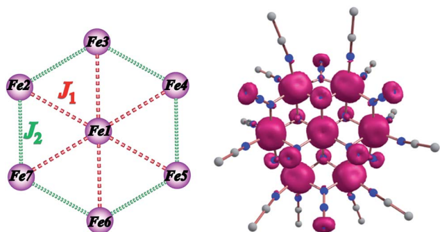
Fig. 5 (left) Magnetic exchange pathways in complex 1; see the text for the DFT computed values. (right) DFT-computed spin-density plots for 1 for which all spins are up, rationalizing the experimental S = 14 ground state. The pink and blue colours represent positive and negative spin densities, respectively.
