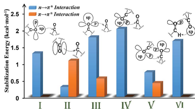
Fig. 8 Plot showing the various orbital interactions in various motifs (I–VI) having CO...CO interactions and the NBO second-order perturbation energy of representative molecules of each motif.
