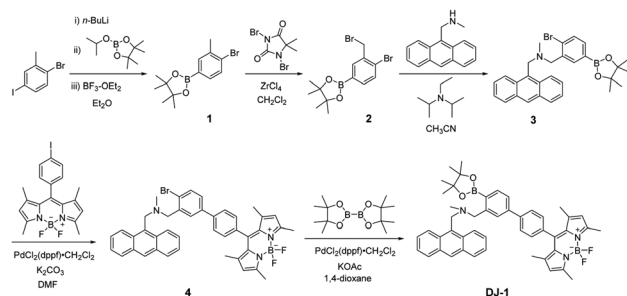
Scheme 1 Synthesis of DJ-1 .
