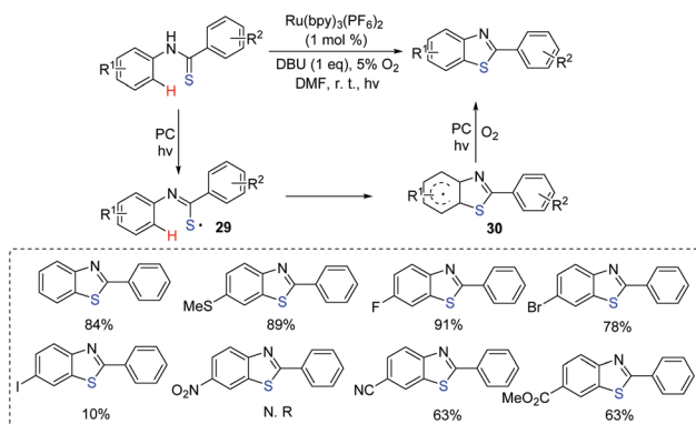
Scheme 14 Synthesis of 2-substituted benzothiazoles.
