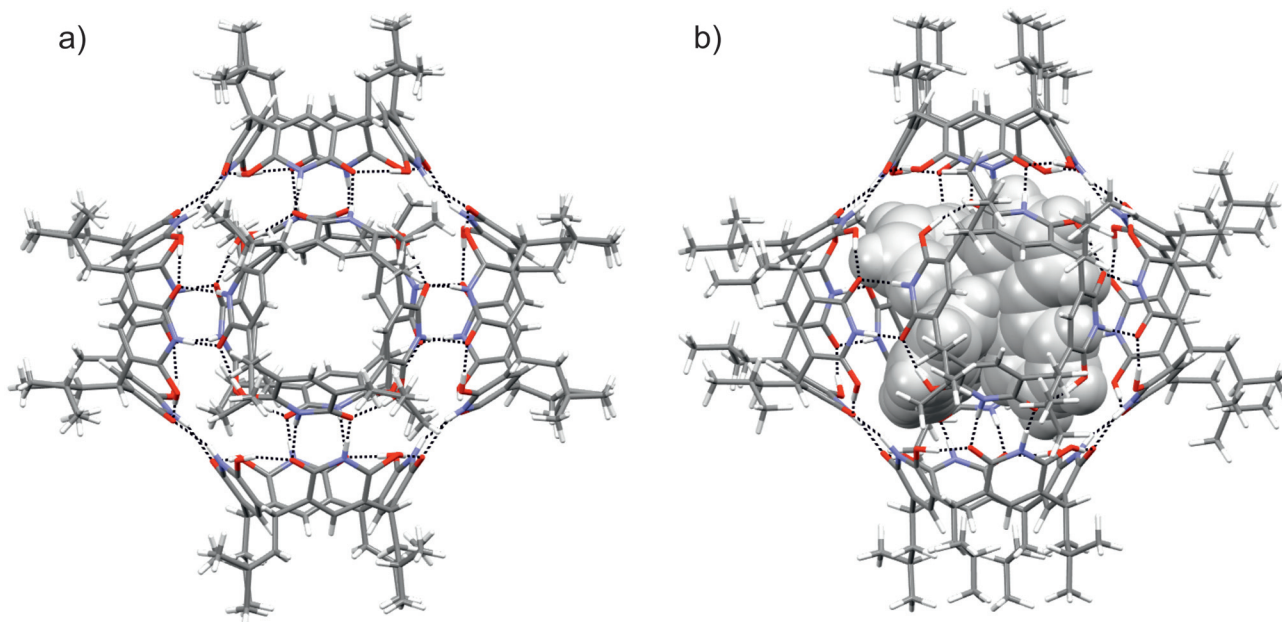
Fig. 3 X-Ray crystal structure of 1 6 and (b) optimized structure of [ 1 6 + G] 2+ at the RI-PBE-D3/def2-SVP level of theory in capped stick model. Tris (bipyridine)-ruthenium(II) (G) is shown in grey CPK model in (b). Black dashed lines represent hydrogen bonds. Color code: H = white, C = grey, N = blue, O = red.
