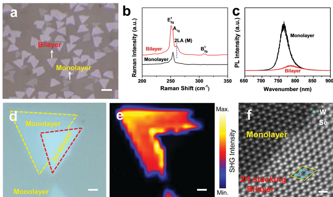
Fig. 1 (a) Optical micrograph of monolayer/bilayer WSe 2 crystals as-grown on a c -plane sapphire substrate. The amount of WO 3 is 0.3 g, while the amount of Se powder is 5.0 g. A high purity of H 2 /Ar is the carrier gas with a fixed flow rate of 5/65 sccm/sccm. The T Se and T WO 3 are maintained at 250 °C and 895 °C, respectively. The growth pressure of the furnace is 10 Torr for the whole CVD growth and the growth time is 15 min; (b) the Raman spectra measurements for monolayer (black) and bilayer (red) WSe 2 crystals; (c) the PL spectra measurements for monolayer (black) and bilayer (red) WSe 2 crystals; (d) optical micrograph of a bilayer WSe 2 crystal with a monolayer WSe 2 crystal as a reference; (e) the corresponding SHG intensity mapping obtained by pixel-to-pixel spatial scanning on the crystals in (d); (f) the HAADF-STEM image for the 2H stacking bilayer WSe 2 crystal (selected from (a)). Scale bars: a, 30 μm; d, 2 μm; e, 2 μm; f, 0.5 nm.
