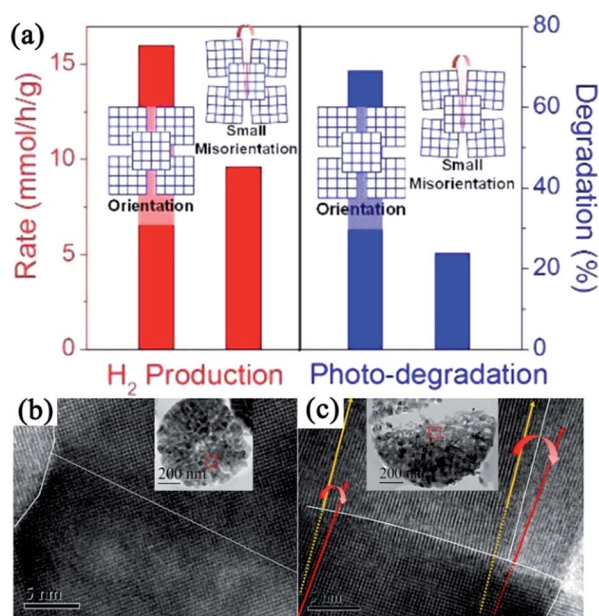
Fig. 4 (a) Schematic illustration of disordered and ordered aggregations of TiO 2 nanoparticles and their corresponding photocatalytic activities. (b) HRTEM image of TiO 2 mesocrystal with oriented orientation. (c) HRTEM image of TiO 2 mesocrystal with misorientation (crystal lattice mismatch). Adapted with permission from ref. 53. Copyright 2015 American Chemical Society.
