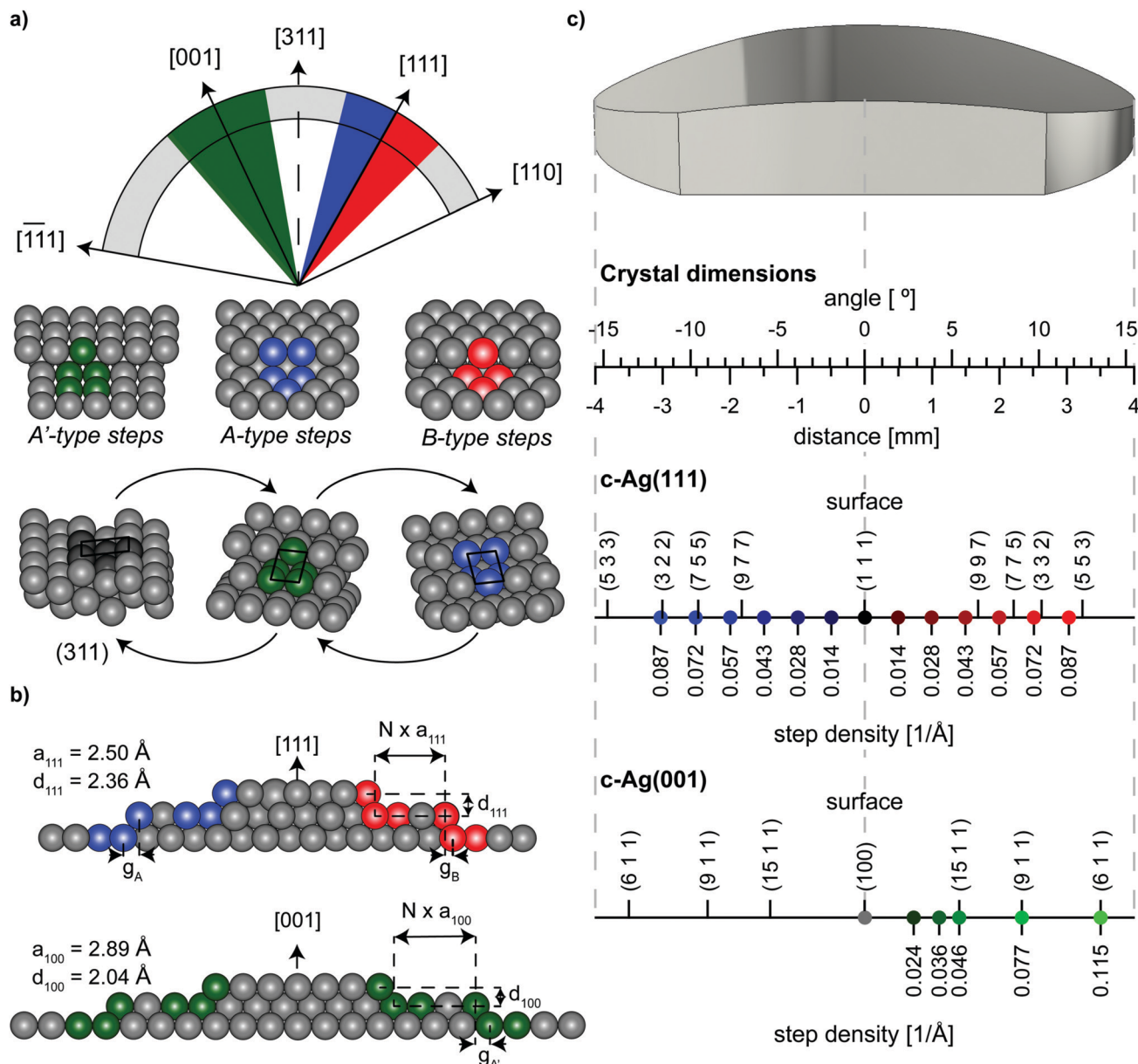
Fig. 1 Schematic drawings of orientation and surface structures of the two curved crystals employed in this study. (a) Orientation of the c-Ag(001)31° \bar{[110]} (green) and c-Ag(111)31° \bar{[110]} (blue and red) crystals on a cylinder with its rotational axis along \bar{[110]} . Below the step types that separate (001)/(111) terraces on the two crystals respectively. Also shown, the (311) surface and its unit cell, and how this surface can be seen as consisting of only A- or only A'-type steps. (b) Schematic microscopic side view of the two crystals, indicating parameters used in eqn (1). In the center, the crystals feature wide terraces. As the crystal curves to the sides, steps are introduced to accommodate the macroscopic curvature. (c) Drawing of the macroscopic shape of the crystals linking macroscopic properties of the crystal (angle of curvature, distance from apex), to microscopic properties found on the surface, i.e. Miller indices of surface structures at specific points of the crystal. Positions of measurements in Fig. 4 are indicated in blue, red, and green with their respective step densities. Step densities for monoatomic steps do not follow the same scale on the two crystals because of different step heights on (001) and (111) terraces, as indicated in (b).
