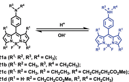
Scheme 16 Fluorescent probes 21a–c for pH.
