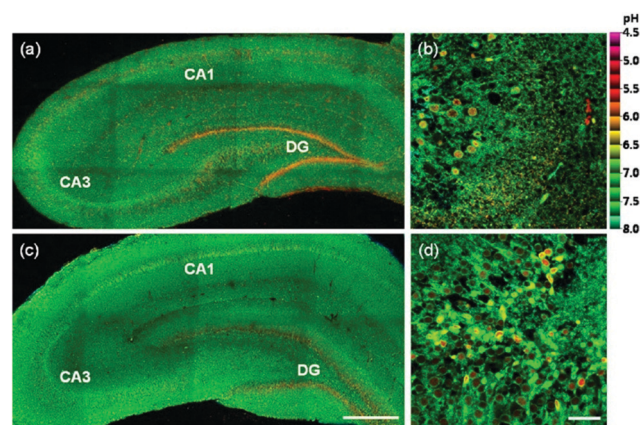
Fig. 43 Pseudocolored ratiometric TPM images ( I_{\text{green}}/I_{\text{IR}} ) of a rat hippocampal slice stained with 30 \mu\text{M} (a and b) 28 and (c and d) 27a . (a and c) 120 \times TPM images along the z-direction at depths of approximately 90\text{--}180 \mu\text{m} were accumulated to visualize the overall pH distribution with 10\times magnification. (b and d) Higher magnification images ( 63\times ) in the regions of DG. Excitation wavelength is 740 nm. Scale bars are (a and c) 300 \mu\text{m} and (b and d) 47 \mu\text{m} . Copyright 2013 American Chemical Society.
