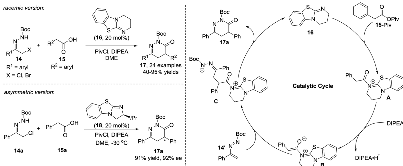
Scheme 7 Isothiurea catalyzed formal [4+2] cycloaddition of azoalkenes with arylacetic acids and the proposed mechanism.
