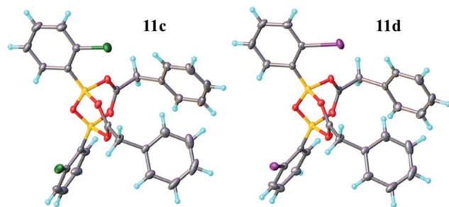
Fig. 6 X-ray structures of B–O–B “ate”-complexes 11c and d.
