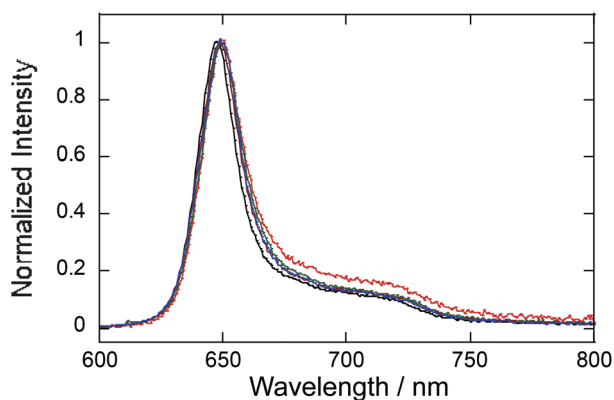
Fig. 3 Phosphorescence emission spectra of PtCP fixed in nano-porous glass with different loading concentrations of 75 \mu\text{M} (blue), 310 \mu\text{M} (green), and 5.2 mM (red) together with PtCP solution in THF (75 \mu\text{M} , black). All samples were deoxygenated by Ar-bubbling.
