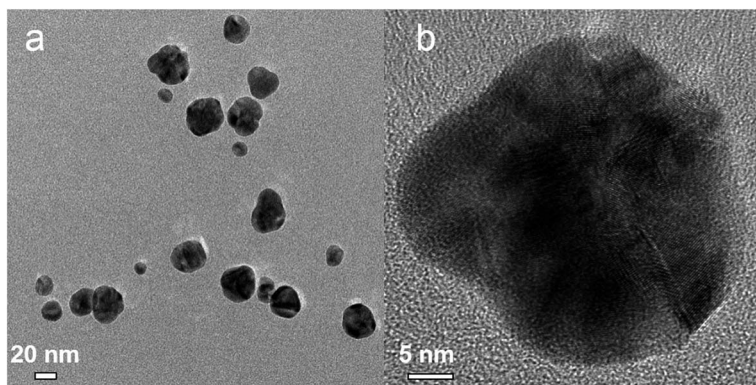
Fig. 13 (a) TEM and (b) HRTEM image for Ag–Pd alloy NPs synthesized by simultaneous reduction of \text{Ag}(\text{NO}_3) and \text{Pd}(\text{NO}_3)_2 with HQ.
