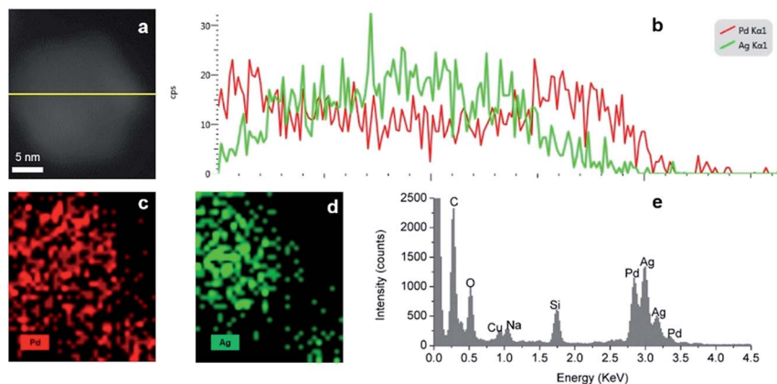
Fig. 14 (a and b) EDS line scan, (c and d) EDS elemental mapping and (e) EDS spectra of Ag–Pd alloy NPs synthesised by simultaneous reduction of \text{Ag}(\text{NO}_3) and \text{Pd}(\text{NO}_3)_2 with HQ.
