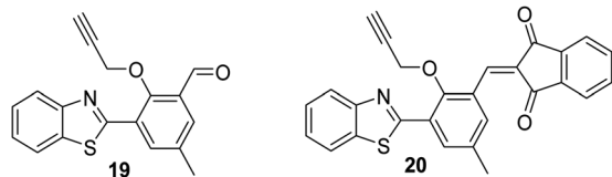
Fig. 4 Two ESPT-based probes 19 and 20 that allow the detection of Pd 2+ . Measurement conditions: HEPES/THF (5 : 2).
