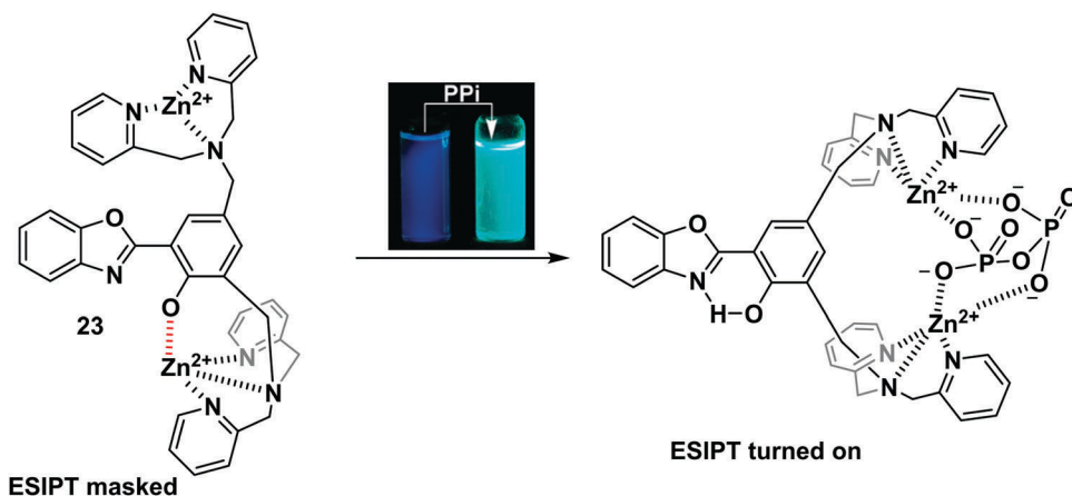
Scheme 22 A binuclear Zn 2+ ESPT based probe 23 for the ratiometric detection of pyrophosphate. Measurement conditions: HEPES buffer (10 mM, pH = 7.4). Reproduced with permission from ( Org. Lett. , 2011, 13 , 1362–1365). Copyright (2011) American Chemical Society.
