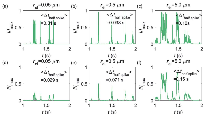
Fig. 7 Chronoamperograms of single enzyme detection at microdisc electrodes featuring radii of 0.05, 0.5 and 5.0 \mu\text{m} . (a–c) are the modelled potentiostat signals after passing a 4 kHz filter, while (d–f) depict the same data filtered via a 50 Hz filter. The average spike duration time for each system is listed on the plot. In the simulation, r_{\text{enzyme}} = 5 \text{ nm} , D_{\text{enzyme}} = 5 \times 10^{-11} \text{ m}^2 \text{ s}^{-1} , D_{\text{P}} = 1 \times 10^{-9} \text{ m}^2 \text{ s}^{-1} , \Delta t_{\text{rw}} = 10^{-6} \text{ s} . The simulation space of d_{\text{enzyme}} is from 5 nm to 5 \mu\text{m} and the total simulation time is 5 seconds.
