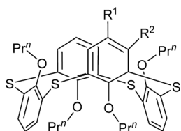
Fig. 80 Structures of compounds 90 – 93 .
