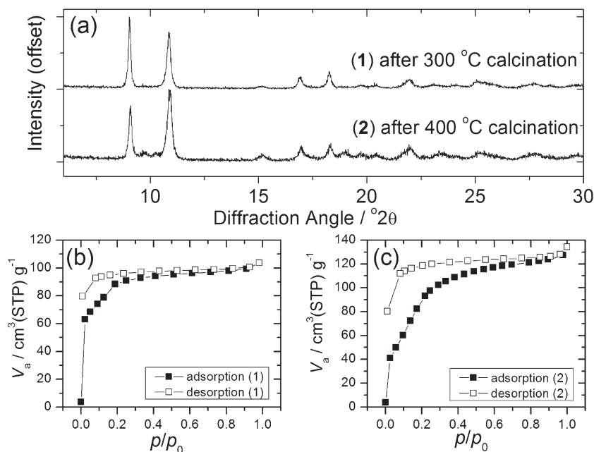
Fig. 6 (a) XRD of Yb 2 (BDC) 3 prepared from (1) and (2) and (b) and (c) BET nitrogen adsorption isotherms of each phase.
