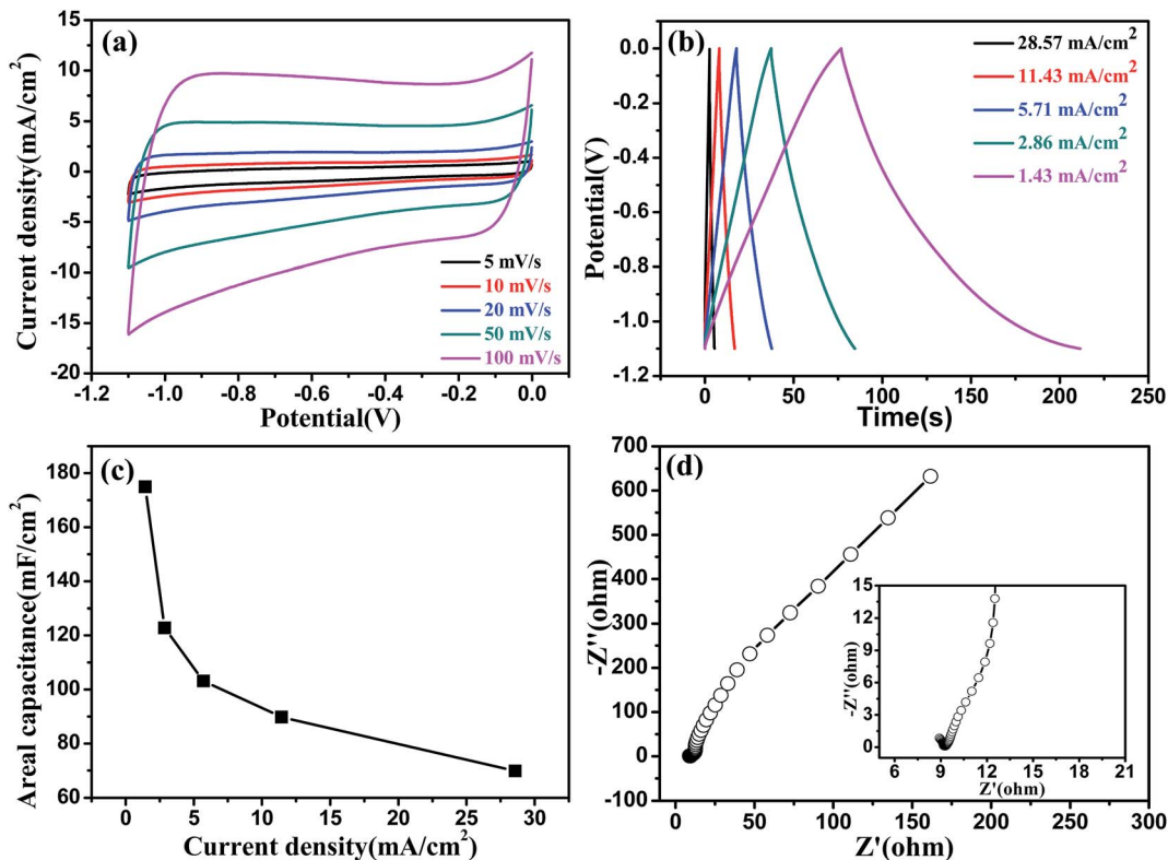
Fig. 4 (a) CV curves at different scan rates; (b) GCD curves at different current densities of the helical MoO 2 in 1.0 M Na 2 SO 4 electrolyte; (c) areal capacitance calculated from GCD curves as a function of current densities; (d) EIS spectra of MoO 2 (inset is the enlarged view of the high frequency region).
