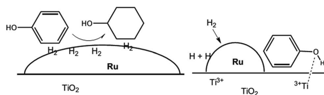
Fig. 3 Illustration of large Ru particles on a TiO 2 support interacting with the aromatic ring and facilitating hydrogenation (left), while small Ru particles create a bifunctional catalyst with the phenyl ring and promote hydrodeoxygenation (right) (adapted from ref. 49).
