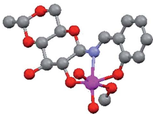
Fig. 2 Structure of 4,6-O-ethylidene- N -(2-hydroxybenzylidene)-β-D-glucopyranosylamine (H 3 L1) derived cis -dioxo Mo(VI) complex. 27
