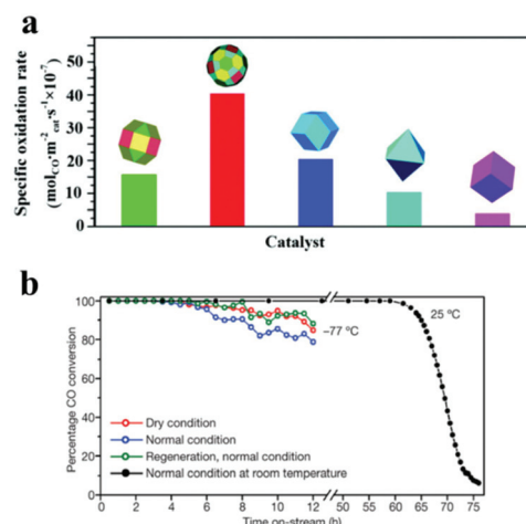
Fig. 8 (a) Specific oxidation rates of the CO oxidation reaction on various shaped \text{Cu}_2\text{O} microcrystals (modified with permission from ref. 38, copyright 2010 American Chemical Society); (b) CO oxidation stability test of \text{Co}_3\text{O}_4 nanorods under stream under different conditions (modified with permission from ref. 22, copyright 2009 Nature Publishing Group).
