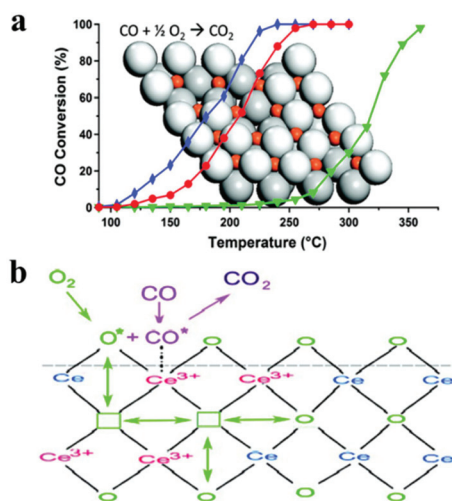
Fig. 7 (a) CO oxidation activity of \text{CeO}_2 NCs post-treated under ambient pressure or vacuum (the blue line presents the activity of nanorods treated under vacuum; the red line presents the activity of nanoparticles treated under vacuum, and the green line presents the activity of nanorods treated under ambient pressure) (modified with permission from ref. 36, copyright 2011 American Chemical Society); (b) scheme of the CO oxidation reaction catalysed by larger \text{CeO}_2 oxygen vacancy clusters (modified with permission from ref. 92, copyright 2009 American Chemical Society).
