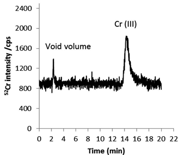
Fig. 9 HPLC-ICP-MS chromatogram of Cr species in mainstream smoke spiked with 1 ng g -1 Cr(VI) (added to the extractant). 0.18 mM, 1 mM EDTA (pH 8) as mobile phase at a flow rate of 0.8 mL min -1 .
