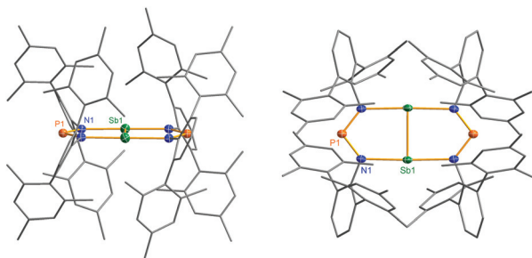
Fig. 11 Molecular structure of 6 (left view: along the Sb–Sb bond, right: topview). Thermal ellipsoids are drawn at 50% probability (173 K). Selected bond lengths [Å] and angles [°]: 6 : Sb1–Sb1' 2.6438(4), Sb1–N1 2.372(2), P1–N1 1.613(2), N1–Sb1–N1' 177.81(9), N1–Sb1–Sb1' 88.91(4), N1–P1–N1'' 104.6(2).
