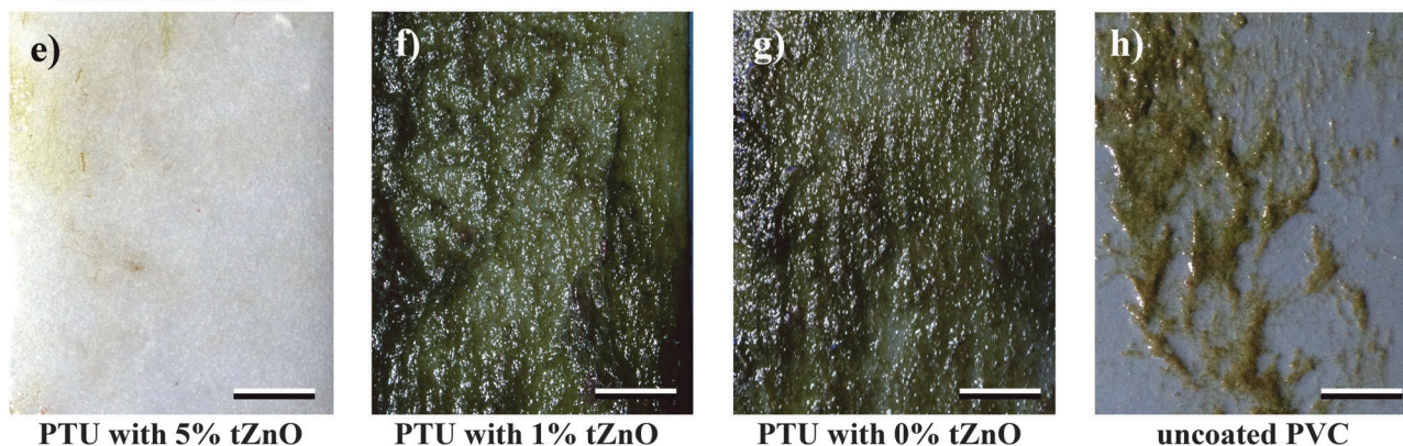
Fig. 4 Preliminary experimental study on three variations of PTU containing (a) and (e) 5 wt% t-ZnO, (b) and (f) 1 wt% t-ZnO and (c) and (g) 0 wt% t-ZnO, (d) and (h) PVC as reference material. Surfaces (a)–(d) were immersed for 20 weeks in the “Pacific sea-tank” at the Aquarium Geomar. Surfaces (e)–(h) were immersed for 30 weeks in the “Baltic sea”-tank at the Aquarium Geomar.
