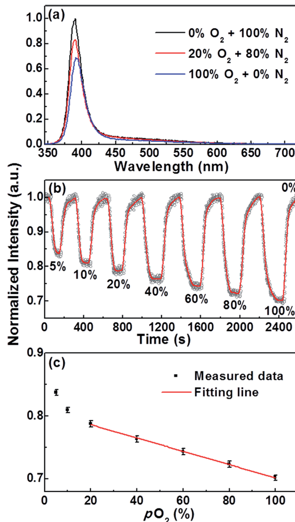
Fig. 4 (a) PL spectra of a TC NR sample measured at T_{NR} = 150 °C in the presence of 100% N_2 , 20% O_2 /80% N_2 and 100% O_2 . (b) Dynamic I_{UV(max)} response of the TC NR sample to various pO_2 at T_{NR} = 150 °C. (c) I_{UV(max)} from the TC NR sample measured as a function of pO_2 at T_{NR} = 150 °C.
