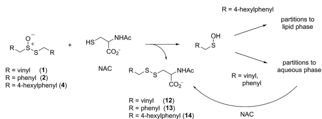
Scheme 3 Alliin and petivericin undergo S -thiolation by NAC to yield sulfenic acids that partition to the aqueous phase where they can react with NAC, whereas hexylated petivericin undergoes S -thiolation to yield a lipophilic sulfenic acid.
