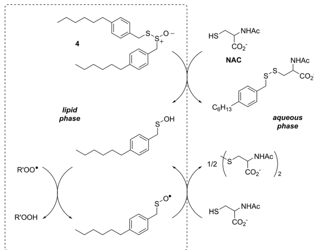
Scheme 1 Proposed mechanism for the RTA activity of 4 observed in the presence of N -acetylcysteine (NAC).
