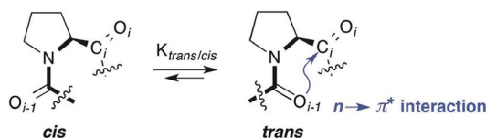
Fig. 1 Trans and cis conformers of Xaa–Pro bonds.
