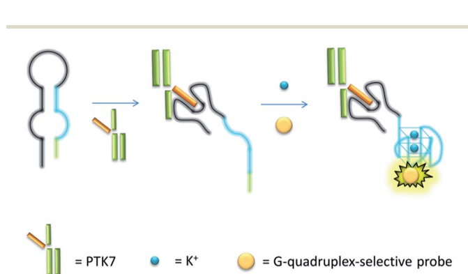
Scheme 1 Schematic representation of the G-quadruplex-based luminescence sensing platform for PTK7 detection.
