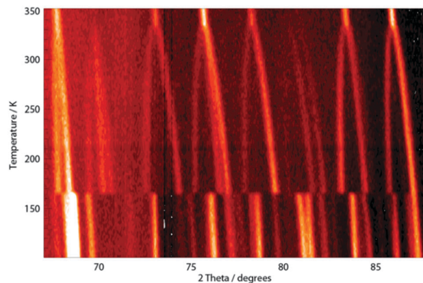
Fig. 3 Stacked plot, viewed vertically, of part of the NPD data (67–88 ° ) collected from MAPbI 3 over the temperature range 100–352 K. Peaks are shown as white and pale orange on a black background. The phase changes at 165 and 327 K are clearly observed as is the overall unit cell expansion.
