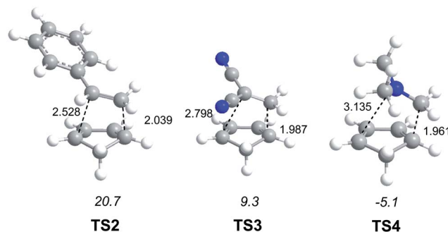
Fig. 2 TSs involved in the DA reactions of Cp 4 with styrene 5 , TS2 , with dicyanoethylene 6 , TS3 , and with iminium cation 7 , TS4 . Relative energies are given in kcal mol –1 , while distances are given in Angstroms.
