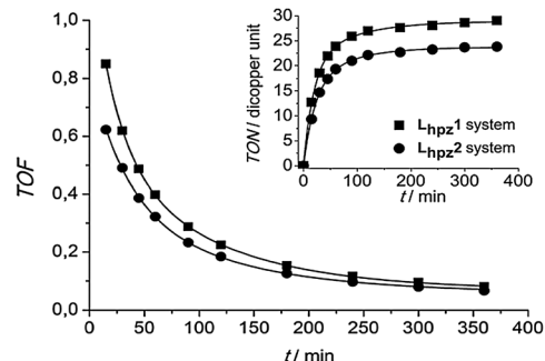
Fig. 2 Turnover frequency as a function of time (15 min < t < 6 hours) for the systems L_{\text{hpz}1} and L_{\text{hpz}2} ; inset: their turnover number per dicopper unit as a function of time.
