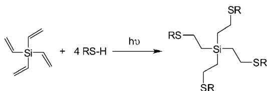
Scheme 12 Synthetic route to 4-armed silanes via photochemical induced thiol-ene coupling with tetravinylsilane.
