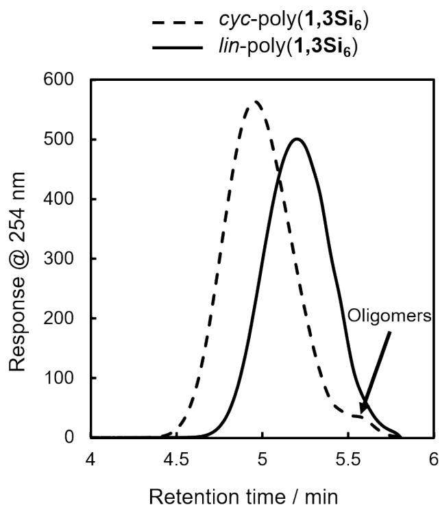
Figure 2. GPC of cyc -poly( 1,3Si 6 ) (dotted line) and lin -poly( 1,3Si 6 ) (solid line). Determined relative to polystyrene standards at 254 nm (THF, [ lin -poly( 1,3Si 6 )] = 1 mg mL -1 , 40 °C, 0.35 mL min -1 , 10 μL injection).
