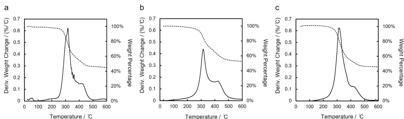
Figure 5. TGA curves of a) lin -poly( 1,4Si 6 ), b) cyc -poly( 1,3Si 6 ) and c) lin -poly( 1,3Si 6 ). Solid lines: derivative weight change; dotted lines: percentage weight change.
