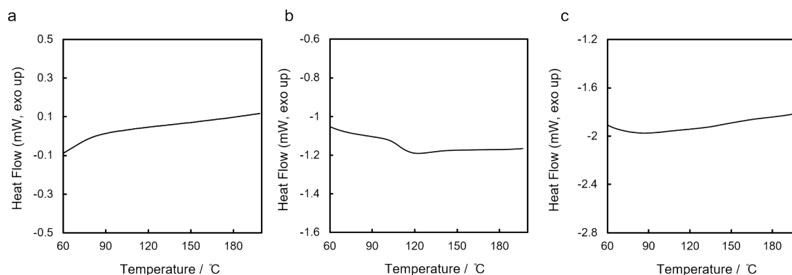
Figure 4. DSC curves of a) lin -poly( 1,4Si 6 ), b) cyc -poly( 1,3Si 6 ), and c) lin -poly( 1,3Si 6 ). The second cycle is shown. Heating rate: 3 °C min -1 for lin -poly( 1,4Si 6 ), 20 °C min -1 for cyc -poly( 1,3Si 6 ) and lin -poly( 1,3Si 6 ).
