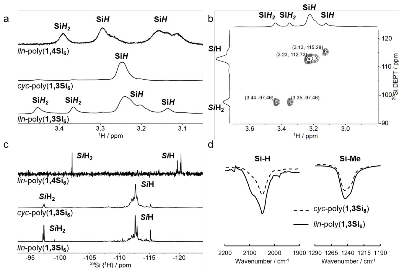
Figure 3. a) Cropped ^1\text{H} NMR spectra of lin -poly( 1,4\text{Si}_6 ), cyc -poly( 1,3\text{Si}_6 ) and lin -poly( 1,3\text{Si}_6 ). Only the SiH region is shown. b) ^1\text{H} - ^{29}\text{Si} HSQC NMR spectrum of lin -poly( 1,3\text{Si}_6 ). Crosspeaks are labelled. c) Cropped ^{29}\text{Si}\{^1\text{H}\} DEPT spectra of lin -poly( 1,4\text{Si}_6 ), cyc -poly( 1,3\text{Si}_6 ) and lin -poly( 1,3\text{Si}_6 ). Only the SiH region is shown. d) Cropped ATR-FTIR spectra of cyc -poly( 1,3\text{Si}_6 ) and lin -poly( 1,3\text{Si}_6 ) highlighting the Si-H and Si-Me regions. HSQC = heteronuclear single quantum coherence; DEPT = distortionless enhancement by polarization transfer.
