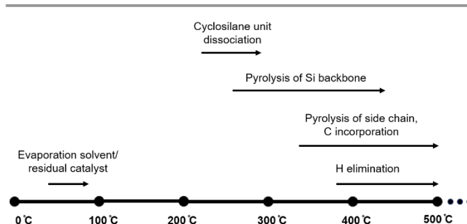
Figure 6. Proposed polycyclosilane pyrolysis.
