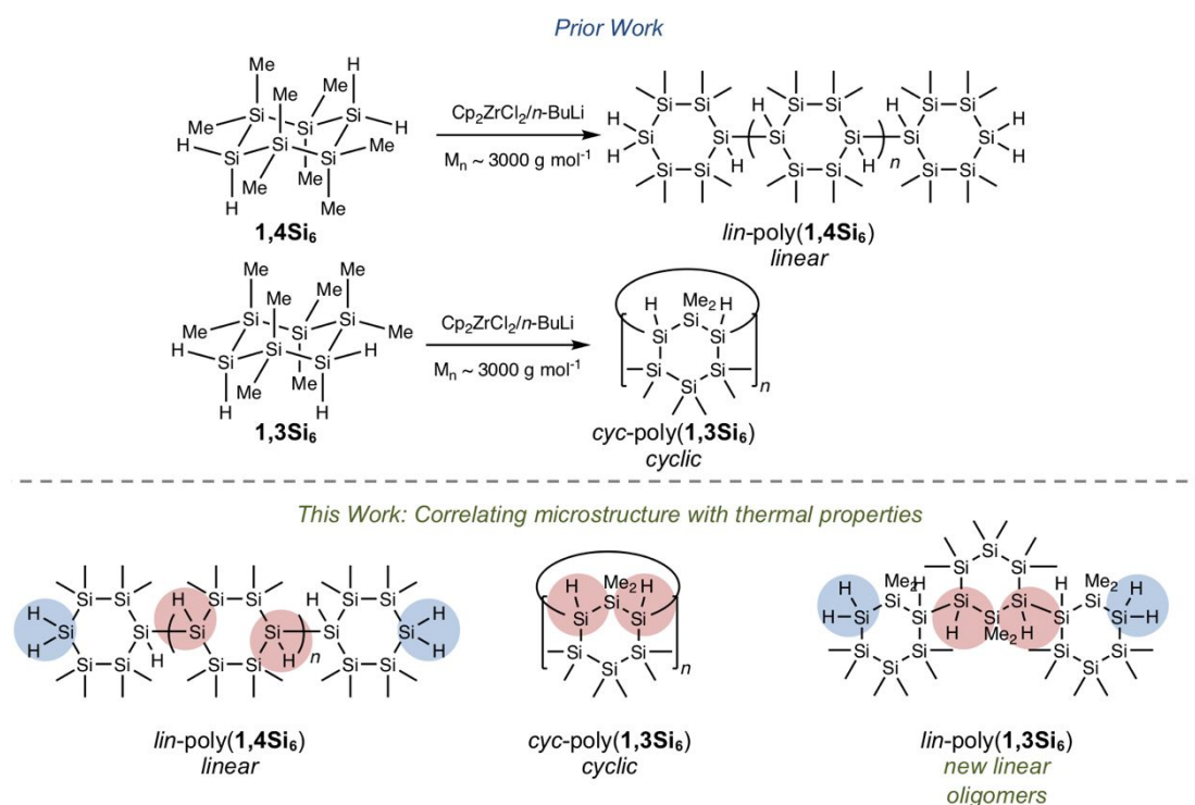
Figure 1. a) Prior work: \text{Cp}_2\text{ZrCl}_2/n\text{-BuLi} -mediated dehydrocoupling polymerization of directional building blocks 1,4Si 6 and 1,3Si 6 . b) This work: Synthesis of new linear lin-poly(1,3Si 6 ) and analysis of relationships between microstructure and thermal decomposition.
