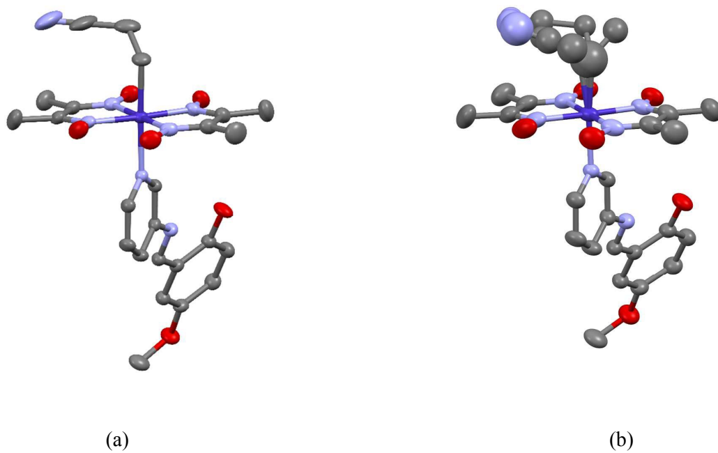
Fig. 11 Molecular structures of III before (a) and after (b) the visible light irradiation. Hydrogen atoms are omitted for clarity. The thermal ellipsoids of atoms are drawn at the 50% probability level.
