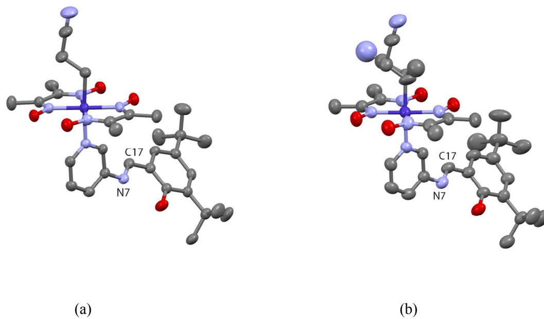
Fig. 9 Major parts of the molecular structures of I before (a) and after (b) visible-light irradiation. The produced 1-cyanoethyl and original 2-cyanoethyl groups take disordered structure in (b). Hydrogen atoms and solvent methanol molecule are omitted for clarity. The thermal ellipsoids of atoms are drawn at the 50% probability level.
