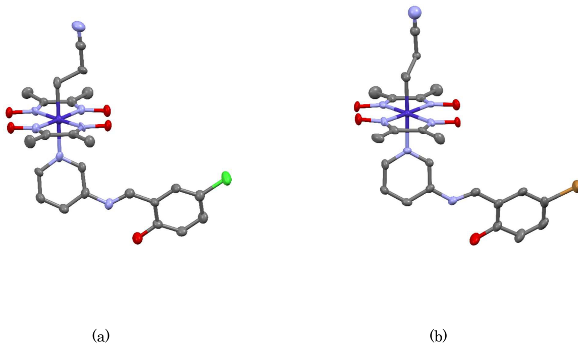
Fig. 13 Molecular structures of IV (a) and V (b). Hydrogen atoms are omitted for clarity. The thermal ellipsoids of atoms are drawn at 50% probability level. Minor part of the 2-cyanoethyl group of V is omitted for clarity.
