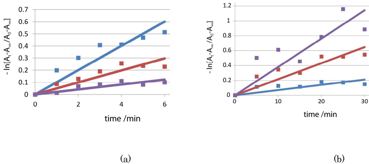
Fig. 7 Fading rates of (a) II and (b) III . The blue line is before irradiation. The red and violet lines are after the 20 and 35 min irradiations in (a), and after the 5 and 10 min irradiations in (b), respectively.
