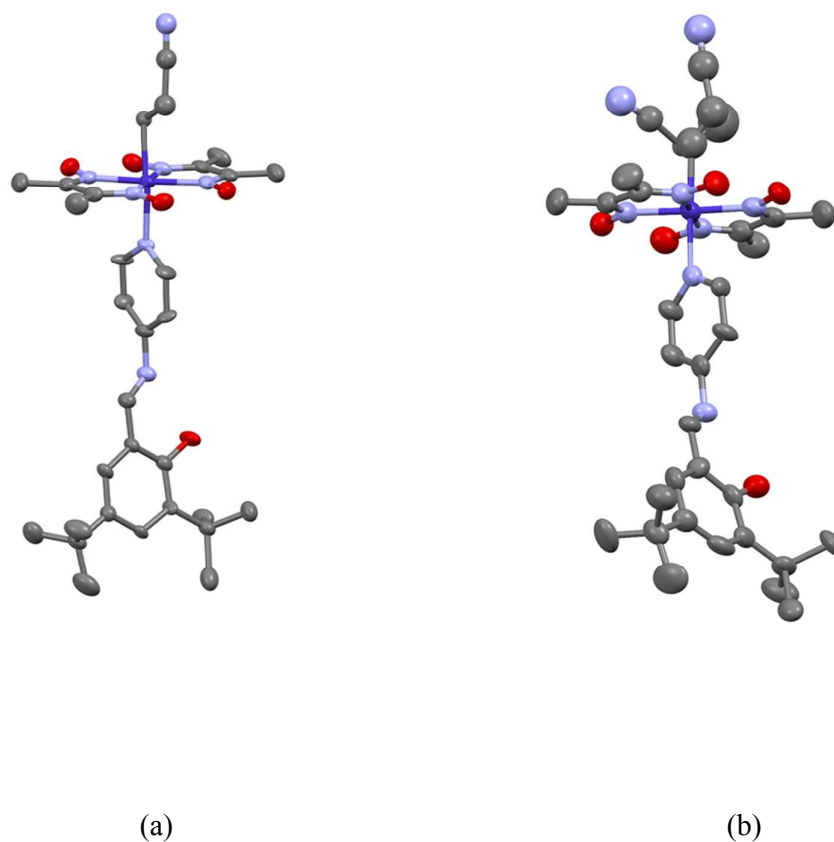
Fig. 10 Molecular structures of II before (a) and after (b) the visible-light irradiation. Hydrogen atoms are omitted for clarity. The thermal ellipsoids of atoms are drawn at the 50% probability level. Minor part of the disordered salicylideneaniline moiety and 2-cyanoethyl group in (a) and salicylideneaniline moiety in (b) are omitted for clarity.
