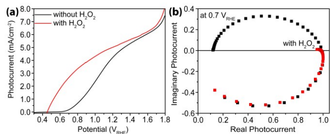
Figure 6. Characterizations with H 2 O 2 as hole scavengers. (a) Steady-state current-voltage curves for sdH with (red) and without (black) H 2 O 2 . (b) IMPS data of sdH with (red) and without (black) H 2 O 2 at 0.7 V vs. RHE.
