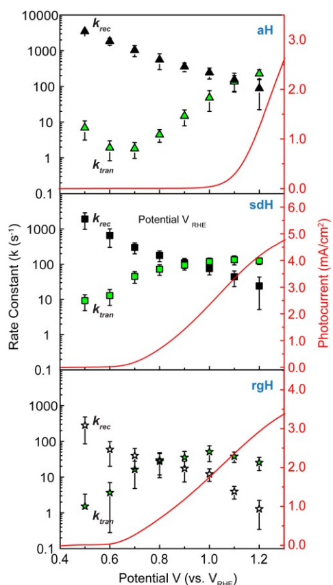
Figure 2. Rate constants extracted from IMPS data at different applied potentials. Top: aH; middle: sdH; and bottom: rgH. Rate constants of recombination are shown as black symbols; rate constants for surface charge transfer are shown as green symbols. The error bar is the standard deviation between different samples (typically 4 to 5 samples are measured for each group of data).
