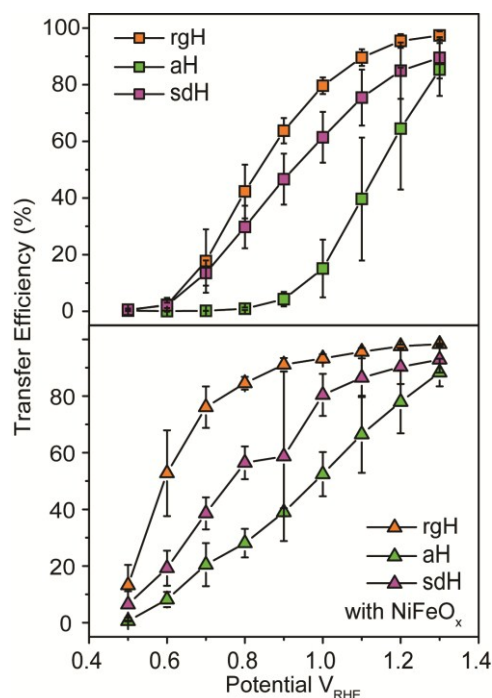
Figure 4. Charge transfer efficiencies for various hematite photoelectrodes without (top panel) and with (bottom panel) NiFeO_x decorations at different applied potentials.
