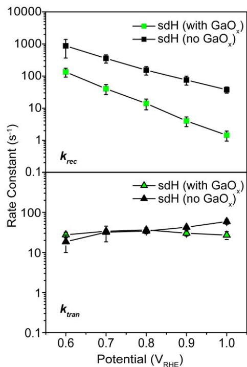
Figure 5. Rate constants for hematite treated with GaO x passivation. Top: recombination; bottom: transfer.
