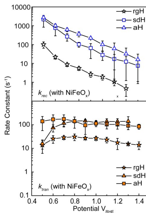
Figure 3. Rate constants for hematite photoelectrodes with NiFeO x surface decorations. Top: Recombination rate constants for photoelectrodes by three different preparation methods; bottom: surface charge transfer rate constants for the same photoelectrodes. The error bars are standard deviations between different samples.
