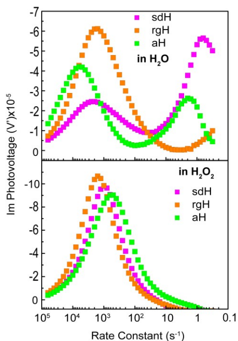
Figure 7. Intensity modulate photovoltage spectroscopy (IMVS) of various hematite photoelectrodes in \text{H}_2\text{O} (top) and in \text{H}_2\text{O}_2 (bottom). Data presented as Bode plots, where the Y axis shows the imaginary component of the complex photovoltage, and the X axis shows the rate constants converted from the modulation frequencies.
