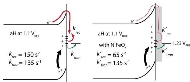
Figure 8. Surface decorations on hematite improves the overall PEC performance by reducing surface recombination. Compared with bare hematite (left), \text{NiFeO}_x does not change k_{\text{tran}} (right). Instead, it reduces the recombination rate constant ( k_{\text{rec}} ) greatly.
