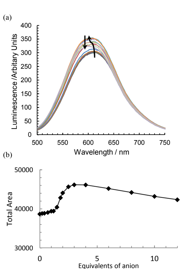
Figure 5 The change in emissive behaviour of a) \{\text{Re}(\text{CO})_3\text{Br}\}_2(\mu\text{-L1}) on the introduction of TBA \text{H}_2\text{PO}_4 and b) the change in integrated area ( \text{CD}_3\text{CN} , 298 K, at approx. 1 \times 10^{-5} \text{ mol dm}^{-3} ).
