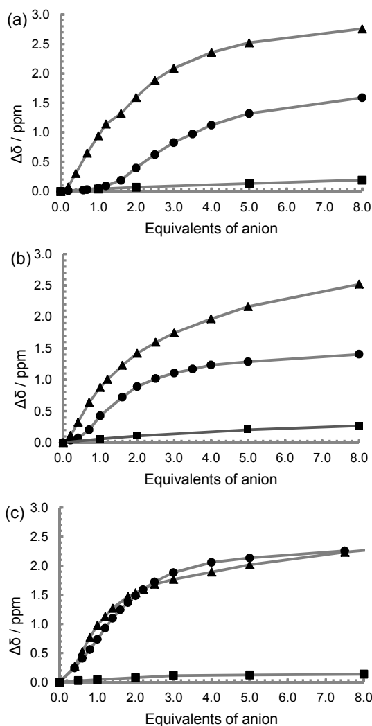
Figure 2 1 H NMR spectroscopic change in NH peak position on the introduction of TBA OAc (▲), TBA Cl (■) and TBA H 2 PO 4 (●); (a) L1, (b) L2, and (c) L3 (50 % DMSO- d 6 / CD 3 CN 400 MHz, 298 K, at approx. 1 \times 10^{-3} mol dm -3 ).
