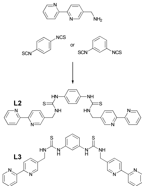
Scheme 2: Synthetic pathway to L2 and L3.
