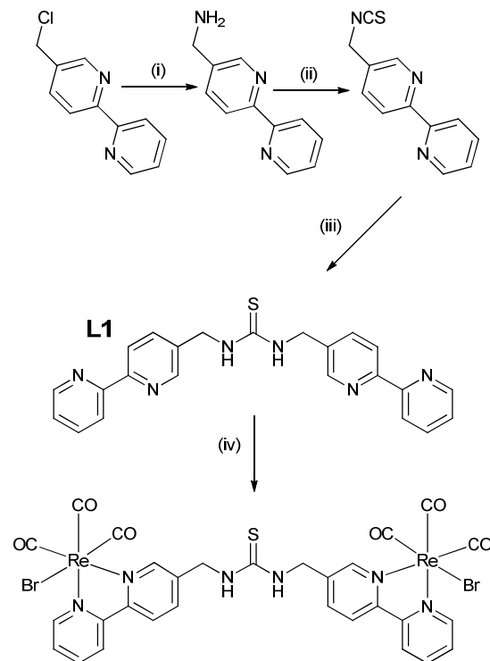
Scheme 1: Synthetic pathway to {Re(CO) 3 Br} 2 (μ-L1); (i) hexamethylenetetraamine, DCM, reflux 16 hrs, then 12M HCl, reflux 16 hrs, (ii) CS 2 , NEt 3 , dry THF stirred for 16 hrs followed by tosyl chloride and stirred for a 16 hrs, (iii) 5-aminomethyl-2,2'-bipyridine, pyridine, reflux 48 hrs, and (iv) [Re(CO) 5 Br], DMSO, 75°C for 16 hrs under N 2 .
