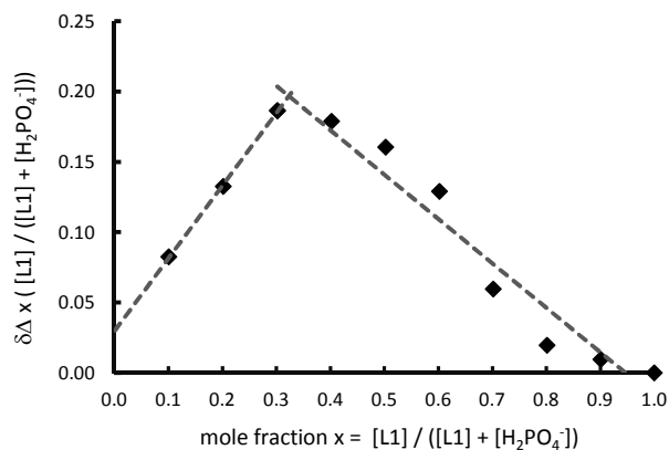
Figure 3 Job plot analysis in the 1 H NMR spectroscopic change in NH peak position on the introduction of TBA H 2 PO 4 (total concentration 1.26 mmol dm -3 , 50 % DMSO- d 6 / CD 3 CN 400 MHz, 298 K, at approx. 1 \times 10^{-3} mol dm -3 ).
