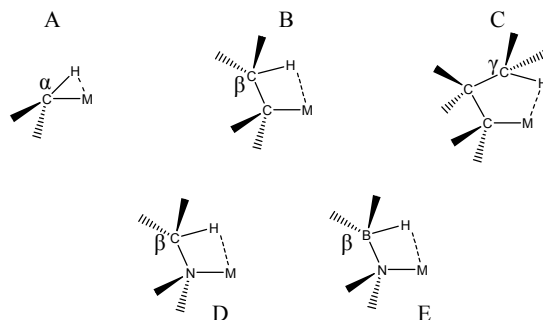
Figure 1: Types of agostic bondings that will be investigated in the present study.
