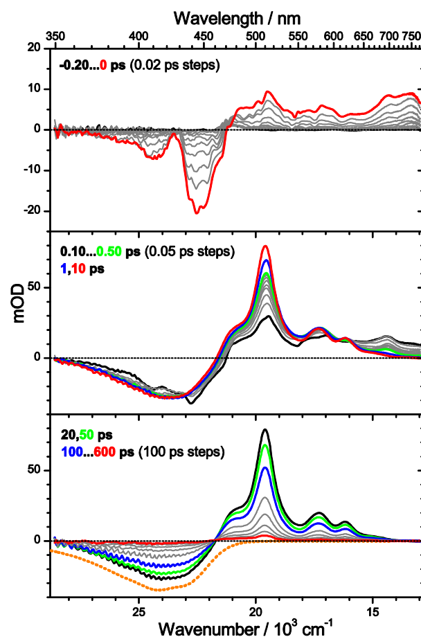
Fig. 6 Transient PSCP absorption spectra of \beta -apo-12'-carotenal in n -hexane for excitation at 490 nm: (upper panel) -0.2...0 ps with 20 fs steps; (middle panel) 0.10...0.50 ps with 50 fs steps, 1 ps and 10 ps; (lower panel) 20 ps and 50 ps, 100...600 ps with 100 ps steps. Selected transient spectra are shown as thick colored lines for guidance. For comparison, the inverted and scaled steady-state absorption spectrum is shown in the lower panel as an orange dotted line.
