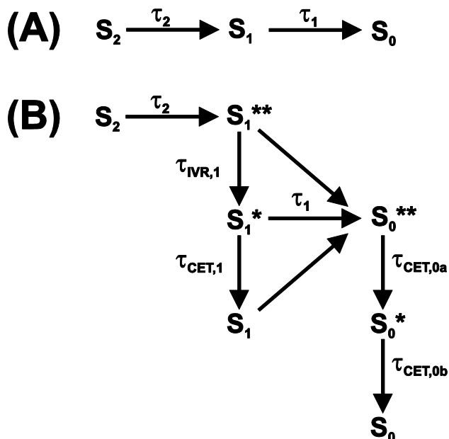
Fig. 1 Two kinetic schemes for the interpretation of carotenoid photophysics. Horizontal and tilted arrows denote electronic transitions between different singlet states, whereas vertical arrows denote intramolecular vibrational redistribution or vibrational cooling by collisional energy transfer to the surrounding solvent.
