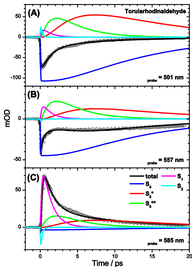
Fig. 9 Kinetic traces for torularhodinaldehyde in n -hexane at (A) \lambda_{\text{probe}} = 501 nm, (B) \lambda_{\text{probe}} = 557 nm and (C) \lambda_{\text{probe}} = 585 nm.
