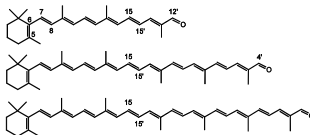
Fig. 2 Chemical structure of \beta -apo-12'-carotenal ( \text{C}_{25}\text{H}_{34}\text{O} , top), \beta -apo-4'-carotenal ( \text{C}_{35}\text{H}_{46}\text{O} , middle) and torularhodinaldehyde ( \text{C}_{40}\text{H}_{52}\text{O} , bottom).
