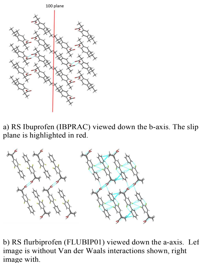
Figure 7. Crystal structures of ibuprofen (IBPRAC) (a) and flurbiprofen (b)
