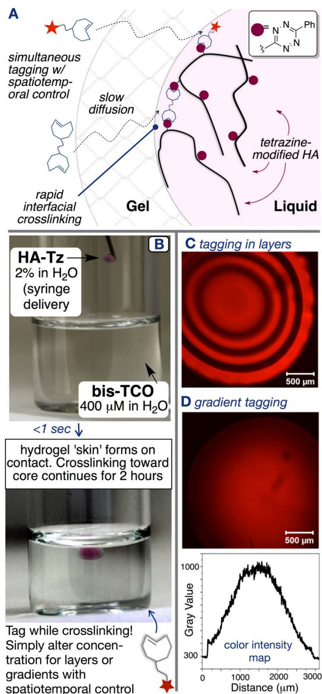
Figure 10. Interfacial bioorthogonal crosslinking. Gel (colorless) interface forms when HA-Tz (pink) contacts a solution of bisTCO. The interfacial kinetics allowed simultaneous introduction of tagging groups (red star in A and B). Spatio-temporal control can be achieved by simply varying the relative concentration of the tagging group as a function of time. (C, D): Confocal images of HA microspheres containing spatially tagged Alexa-TCO (red) in an onion-like layered structure (C) or in a radial gradient (D). 80
