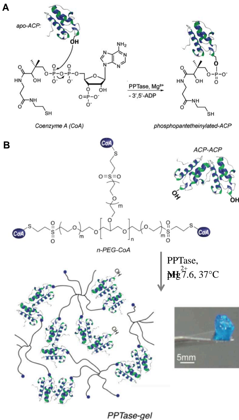
Figure 11. (A) General mechanism of phosphopantetheinyl transferase (PPTase)-catalyzed transfer of phosphopantethein prosthetic group of CoA to the serine residue of ACP; (B) Hydrogel formed between branched PEG-CoA and fluorescent ACP fusion protein. 212
