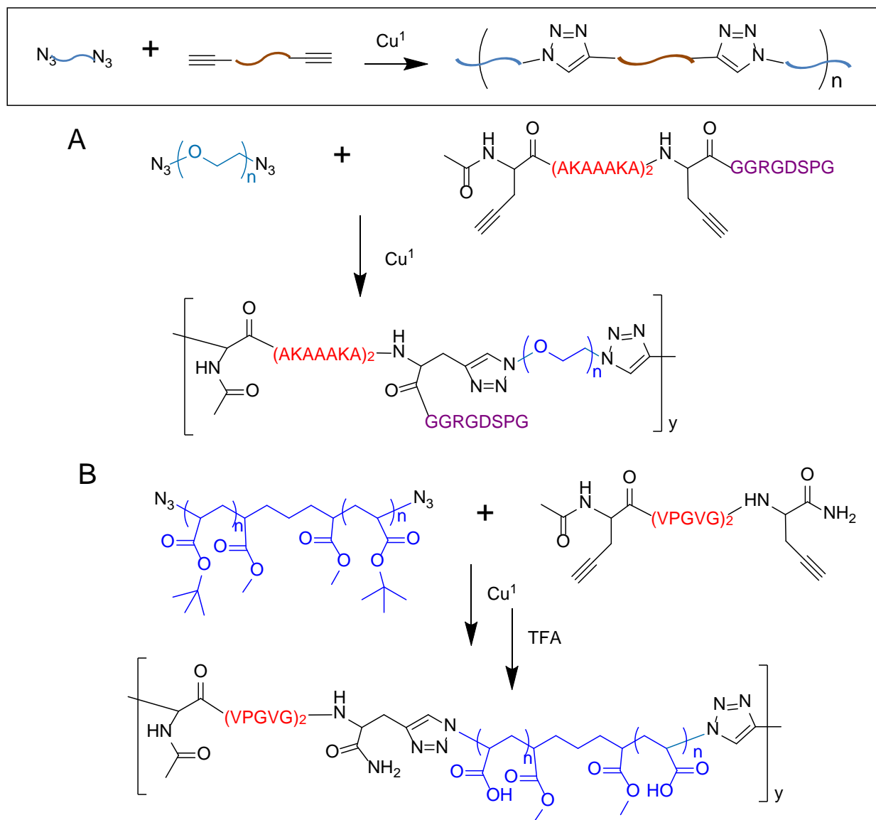
Figure 2. Elastin-mimic hybrid multiblock copolymers synthesized using CuAAC chemistry. (A): Multiblock copolymers contain (AKAAAKA) 2 sequence for crosslinking and GGRGDSPG for cell adhesion. (B): The peptide sequence (VPGVG) 2 is adopted from elastin that contributes to elasticity. 91-93
