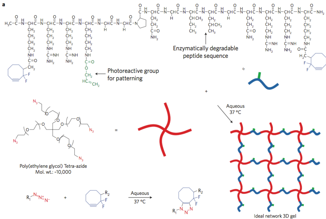
Figure 12. Two independent orthogonal chemistries were applied to the preparation of the PEG/peptide network. The initial gelation was induced by SPAAC and subsequent spatial patterning was achieved using thiol-ene photocoupling chemistry. 145
