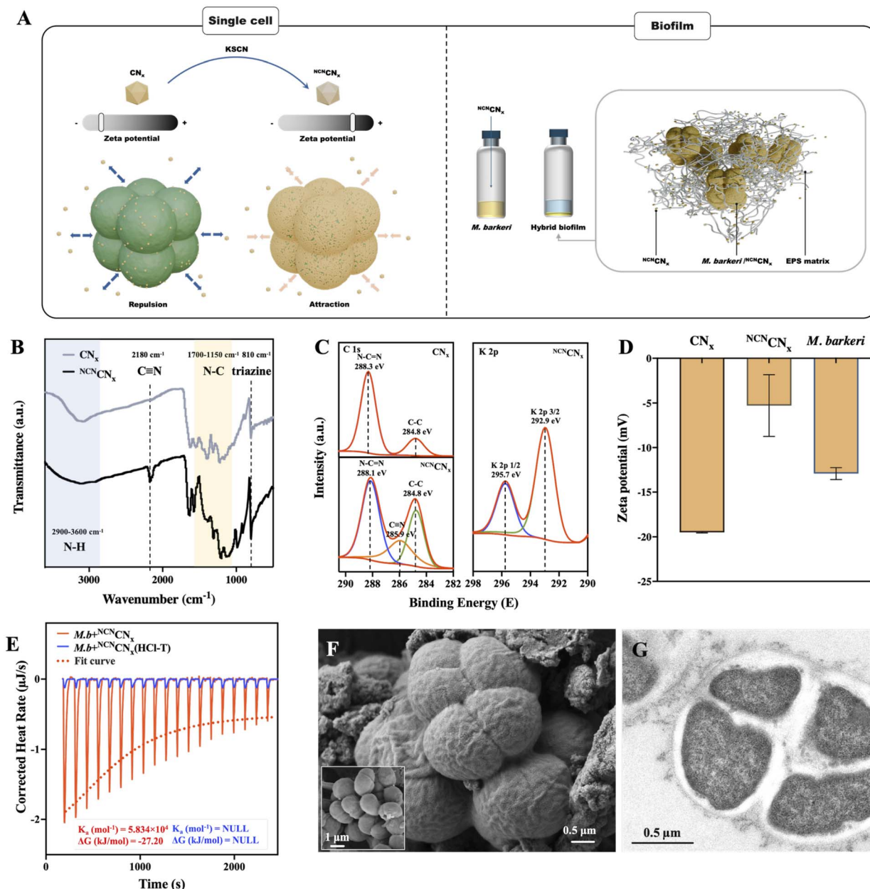
Fig. 1 Formation of hybrid biofilms. (A) Schematic illustration of hybrid single cells and hybrid biofilms. (B) FTIR spectra of \text{CN}_x and \text{N}^{\text{CN}}\text{CN}_x . (C) C 1s and K 2p XPS spectra of \text{CN}_x and \text{N}^{\text{CN}}\text{CN}_x . (D) Zeta potential of \text{CN}_x , \text{N}^{\text{CN}}\text{CN}_x , and M. barkeri . (E) Real-time ITC thermograms for the interactions of M. barkeri with \text{N}^{\text{CN}}\text{CN}_x and with acid-treated \text{N}^{\text{CN}}\text{CN}_x . (F) SEM image of the \text{N}^{\text{CN}}\text{CN}_x / M. barkeri surface (the inset image shows bare M. barkeri ). (G) TEM image of \text{N}^{\text{CN}}\text{CN}_x / M. barkeri .
