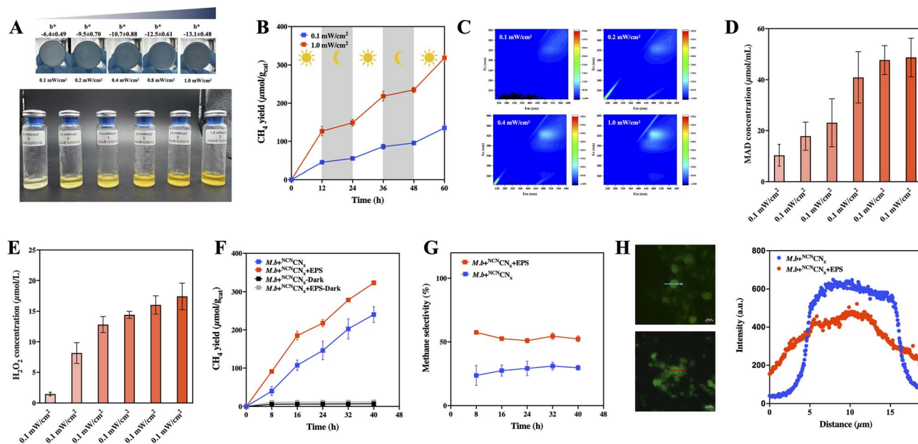
Fig. 3 Optical properties of hybrid biofilm systems under illumination, photodamage of biofilms, and the protective role of EPSs in hybrid biofilms. (A) Top: the biofilm at the bottom of the bottle turns blue under light (the inset numbers represent the mean CIE b^* values derived from digital colorimetric analysis, quantifying the intensification of the blue color). Bottom: the supernatant of the hybrid system turns yellow under light. (B) Methane production under light/dark cycles. (C) 3D-EEM analysis of the supernatant at varying light intensities. (D) MDA concentration at different light intensities. (E) \text{H}_2\text{O}_2 concentration at different light intensities. (F) Methane production under EPS addition. (G) Methane selectivity under EPS addition. (H) Left: fluorescence microscopy image of DCFDA-labeled cells. Right: fluorescence intensity at the marked positions on the fluorescent image.
