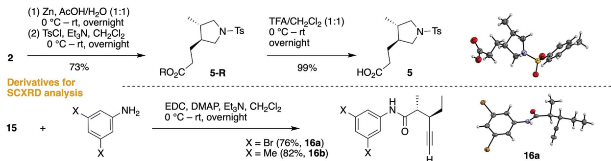
Fig. 4 Synthesis of the AD half (upper panel) and the BC half (middle panel). The preparation of derivatives and resulting single-crystal X-ray structures (lower panel) validated the desired trans -dialkyl stereochemistry in each case.
