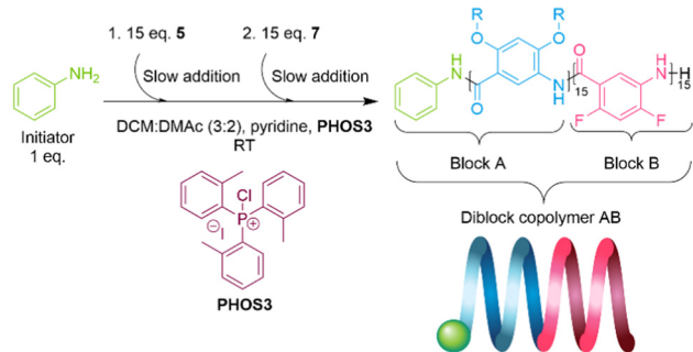
Scheme 2 Top: Synthetic paths for monomers 5 and 7 . (a) K_2CO_3 , DMF, 15-bromo-2,5,8,11-tetraoxapentadecane 2 , 51%. (b) H_2/Pd/C , MeOH, EtOAc, quant. (c) KOH, EtOH, 60%. (d) H_2/Pd/C , MeOH, EtOAc, quant. Bottom: Polymerization conditions of diblock copolymer AB.
