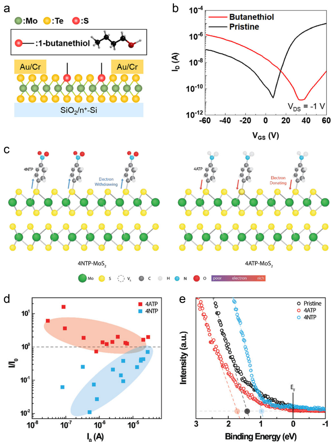
Fig. 2 Surface charge-transfer mechanisms for molecular doping of 2D TMDs. (a) Schematic illustration of 1-butanethiol molecular adsorption on monolayer \text{MoTe}_2 , forming surface dipoles that withdraw electrons from the channel. (b) Transfer characteristics of \text{MoTe}_2 FETs before and after butanethiol functionalization, showing a positive V_{th} shift and enhanced p-type conduction. (c) Schematic models of 4-aminothiophenol (4ATP, electron-donating) and 4-nitrothiophenol (4NTP, electron-withdrawing) adsorption on \text{MoS}_2 , illustrating opposite charge-transfer directions. (d) Statistical I_{on}/I_{off} ratios comparison demonstrating p-type conversion with 4ATP and n-type reinforcement with 4NTP. (e) Ultraviolet photoelectron spectra (UPS) confirming the Fermi-level upshift (4NTP) and downshift (4ATP) via interfacial dipole modulation. Reproduced from ref. 35 (panels a and b) and ref. 36 (panels c–e) under the Creative Commons Attribution License (CC BY 4.0).
